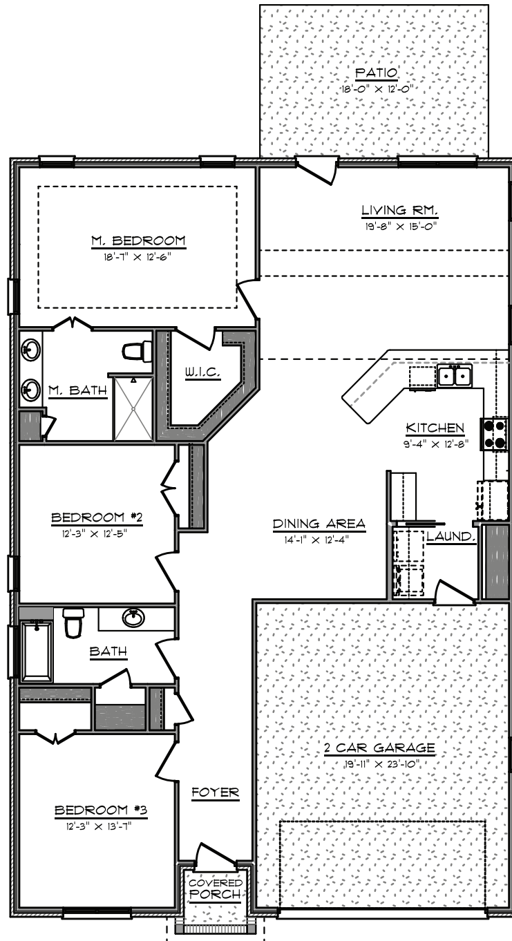
FIRST FLOOR PLAN SPACE 1901 SQUARE FOOT
